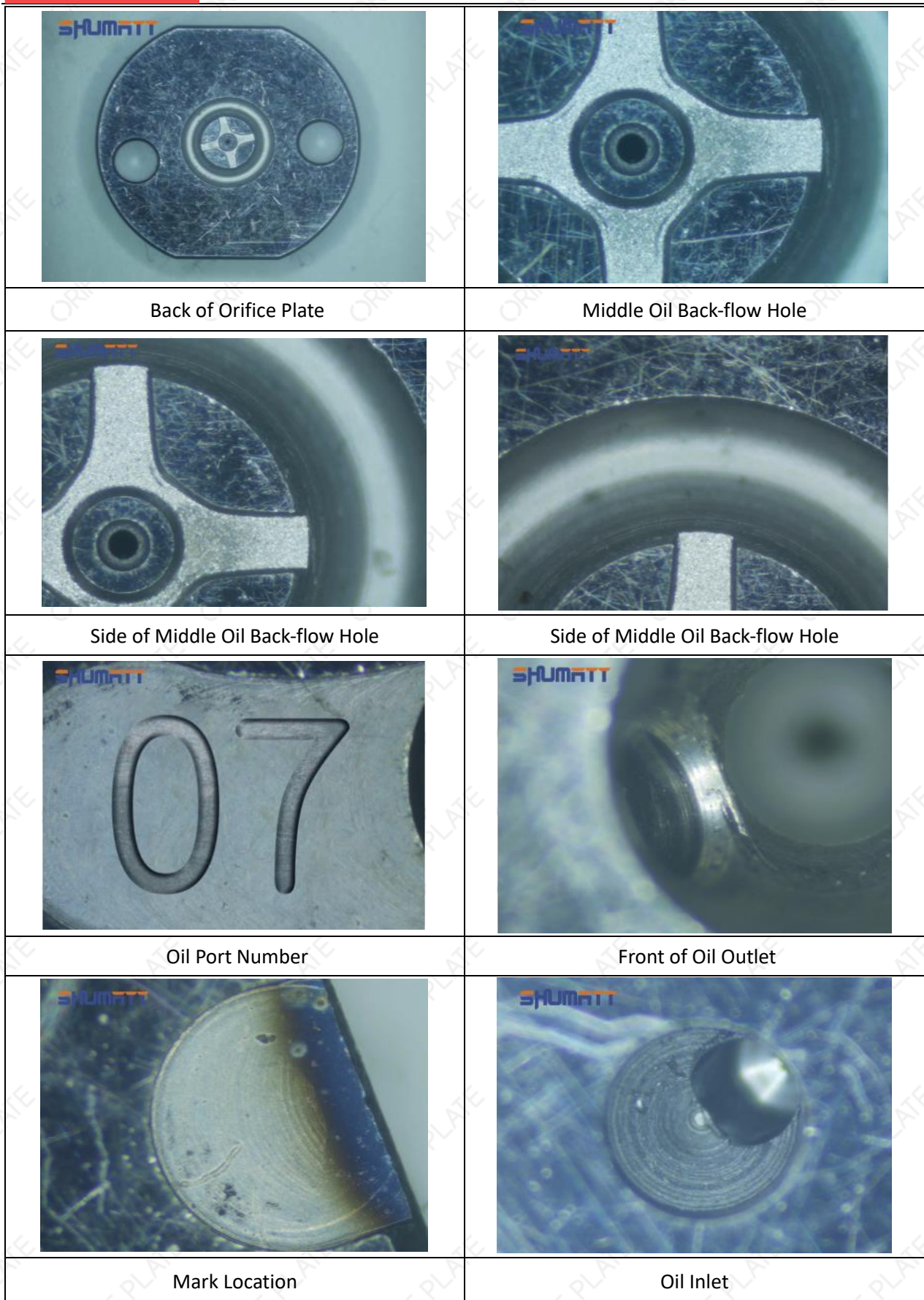
(4) 095000-7530 Injector Orifice Plate 07# Neutral Orifice Plate's Multi-angle Pictures
